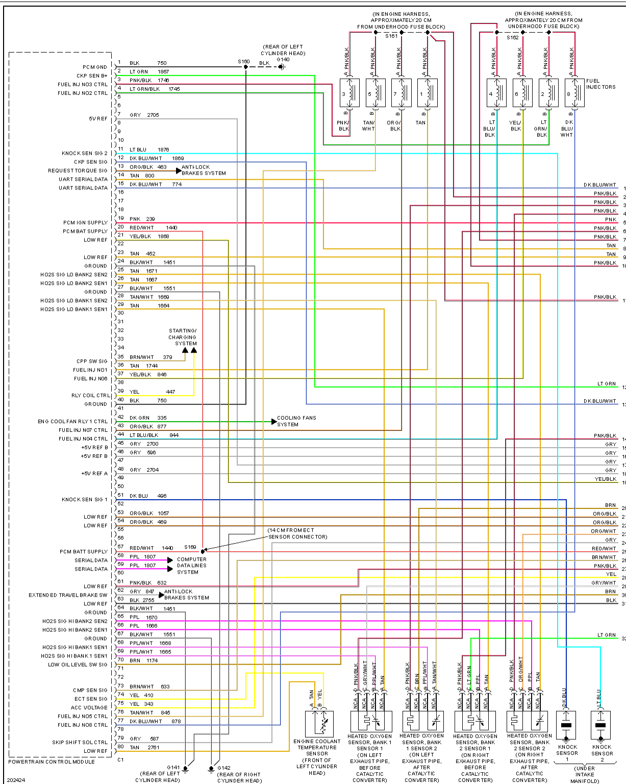
Fig. 26: 5.7L VIN S, Engine Performance Circuit (1 of 4)
