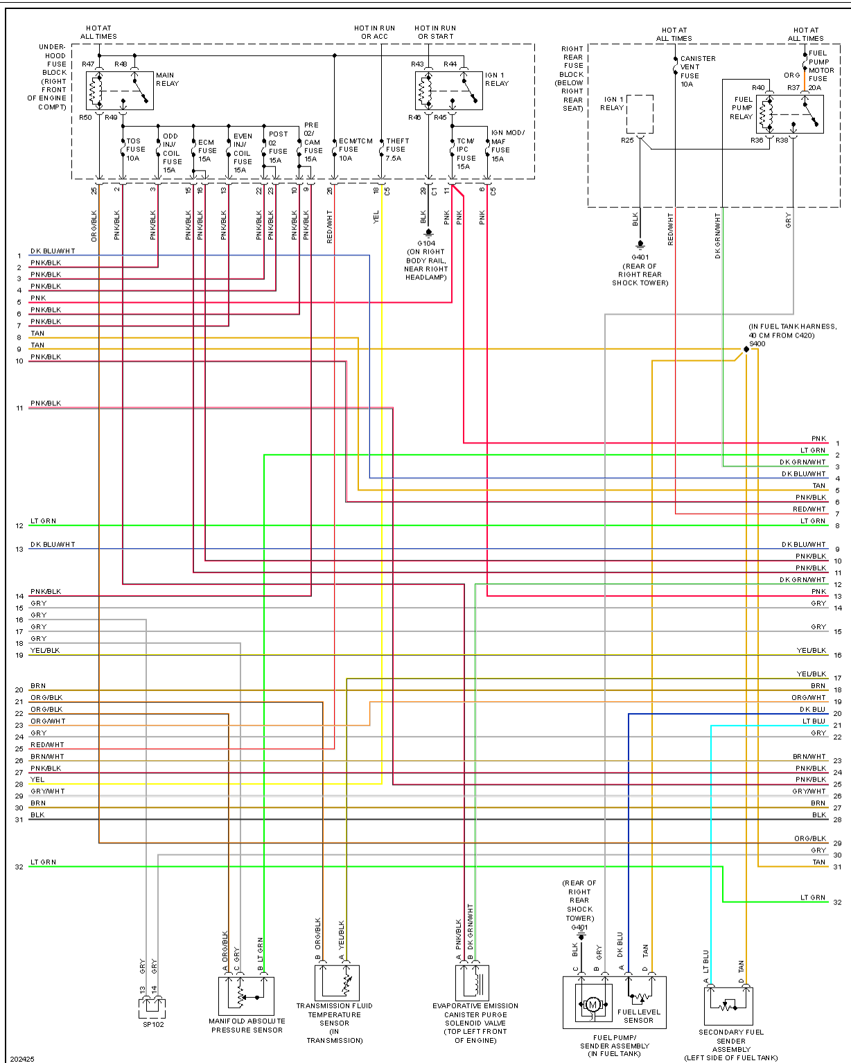
Fig. 27: 5.7L VIN S, Engine Performance Circuit (2 of 4)
